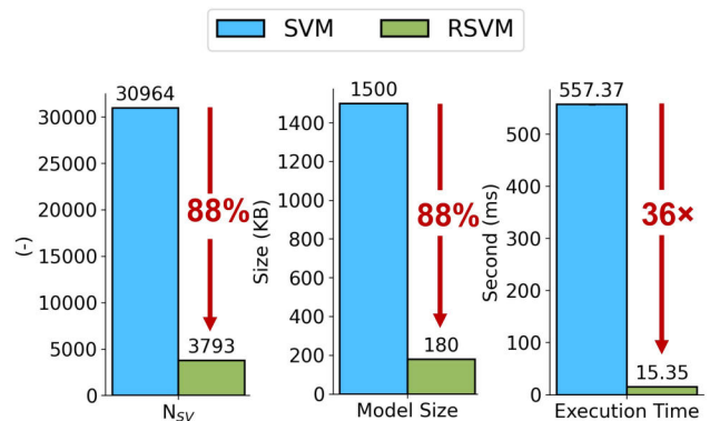
Fig. 4. The comparison of RSVM and SVM model property.
